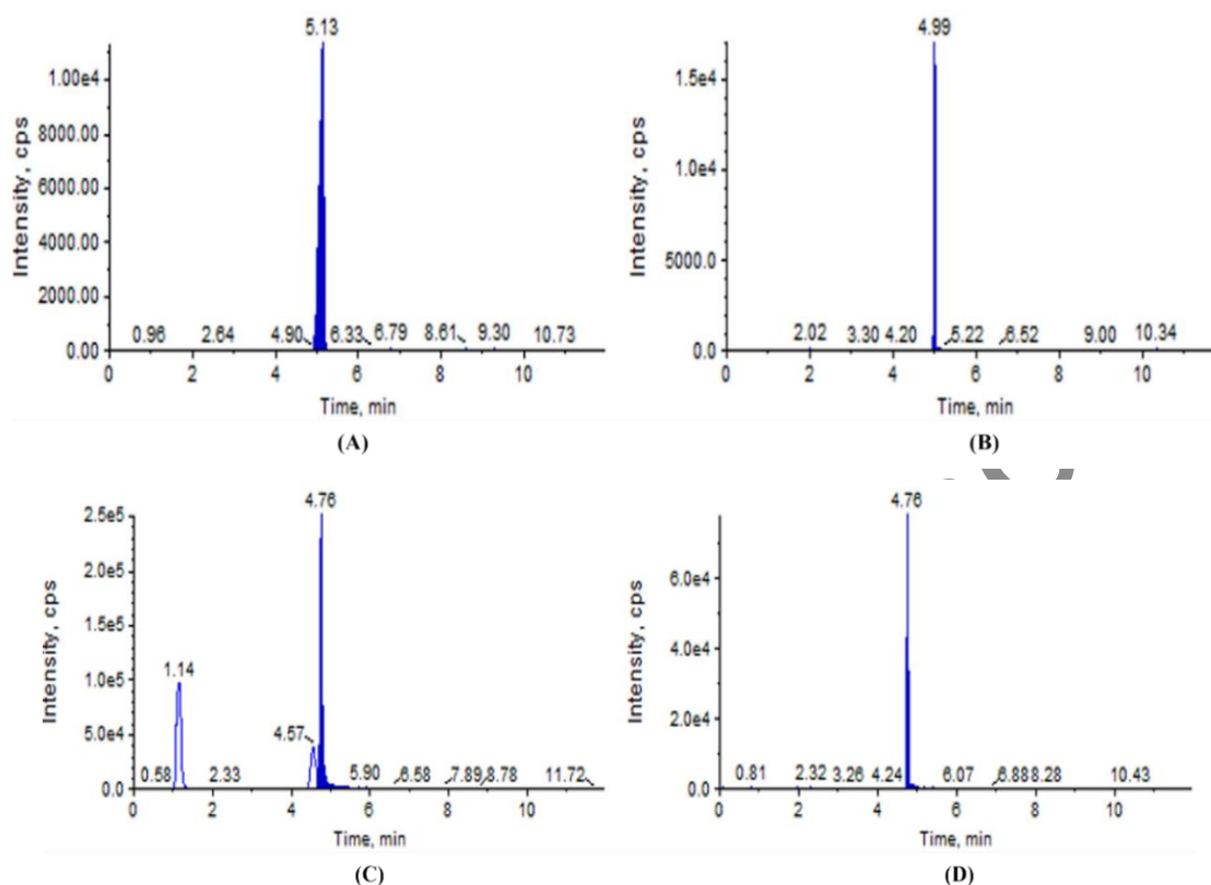
Figure 1. Chromatograms of erythromycin with two mobile phase systems: (A) 0.1% formic acid + 10 mM \text{NH}_4\text{HCO}_2/\text{ACN} , (B) 0.1% formic acid/ACN, and of enrofloxacin with two mobile phase systems: (C) 0.1% formic acid + 10 mM \text{NH}_4\text{HCO}_2/\text{ACN} , (D) 0.1% formic acid/ACN.
